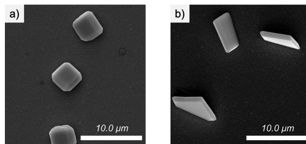
Figure 1. a, b) SEM images of single m- \text{BiVO}_4 crystals with different morphologies synthesized on FTO substrate. The morphology was altered by changing the ramp rates during hydrothermal synthesis from 298 K to 433 K. The m- \text{BiVO}_4 crystal in (a) and (b) are denoted BV01 and BV02, respectively.
